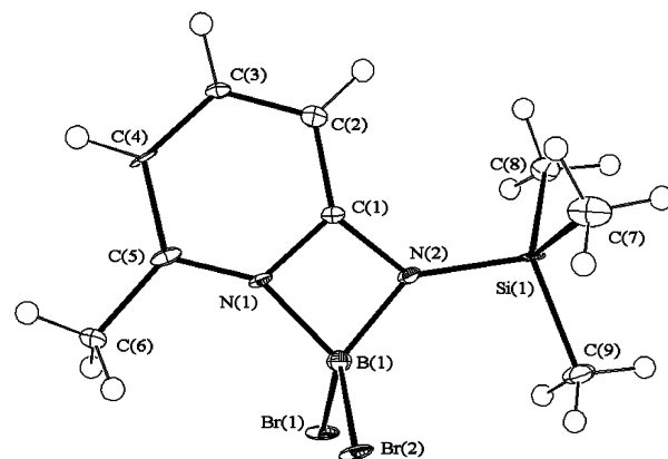
Fig. 1 Molecular structure of 1c , with ellipsoids drawn at the 50% probability level.
