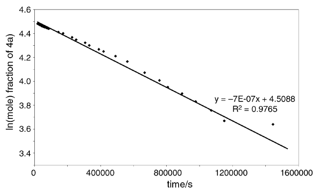
Fig. 5 Plot of \ln(\text{mole fraction of } \mathbf{4a}) vs. time for the thermolysis of 4a at 55^\circ\text{C} , as determined from integration of ^1\text{H} NMR signals. †
