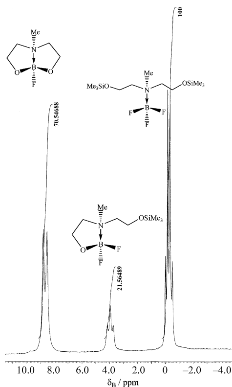
Fig. 6 11 B{ 1 H} NMR signals for 8a , 9a and 10a in benzene at 55^\circ\text{C} .
