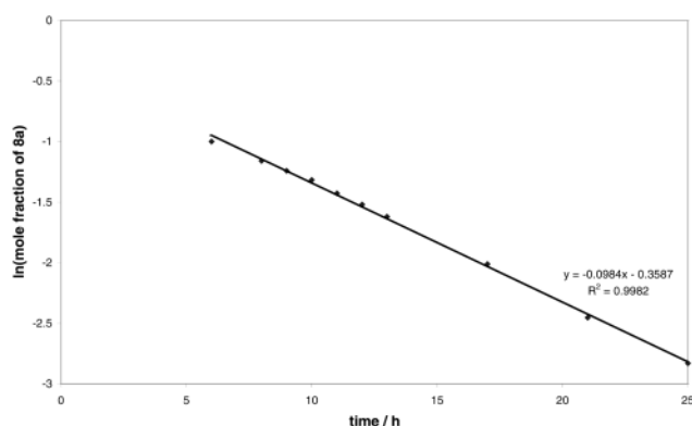
Fig. 8 Plot of \ln(\text{mole fraction of } \mathbf{8a}) vs. time for the thermolysis of 8a at 55 °C, as determined from integration of ^{11}\text{B} NMR signals.§
