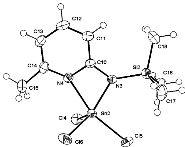
Fig. 3 Molecular structure of one of the two independent molecules of 3 , with ellipsoids drawn at the 50% probability level.
