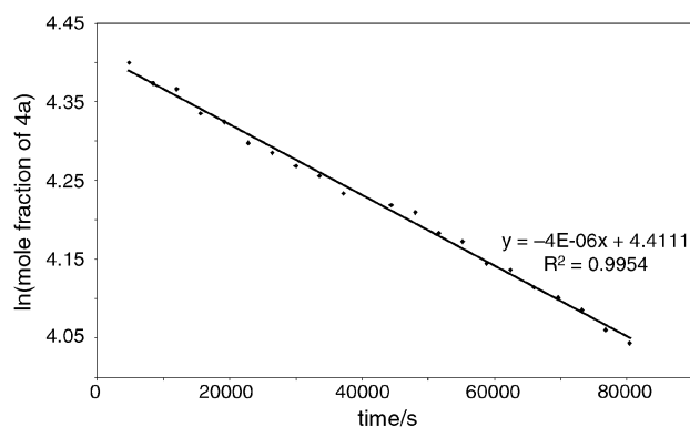
Fig. 4 Plot of \ln(\text{mole fraction of } \mathbf{4a}) vs. time for the thermolysis of 4a at 75^\circ\text{C} , as determined from integration of ^1\text{H} NMR signals. †
