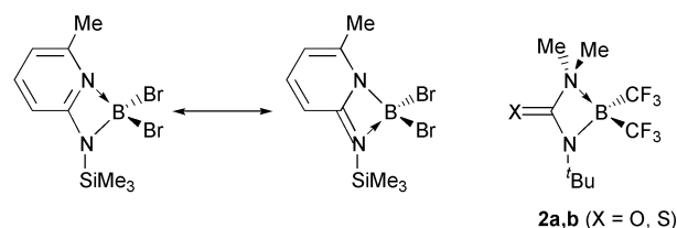
Fig. 2 Proposed 'diaza-allyl' formulation for 1c .
