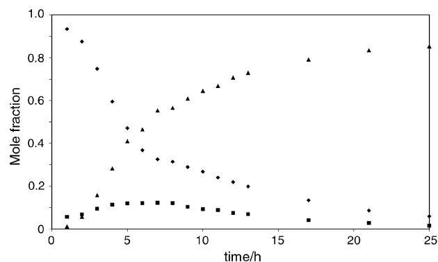
Fig. 7 Plot of mole fraction vs. time for compounds 8a (diamonds), 9a (squares) and 10a (triangles) during the thermolysis of 8a at 55 °C (as determined from integration of ^{11}\text{B} NMR signals).§
