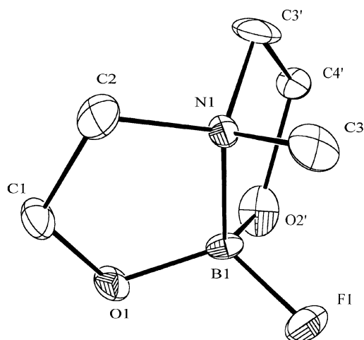
Fig. 9 Molecular structure of 10a , with ellipsoids drawn at the 30% probability level.
